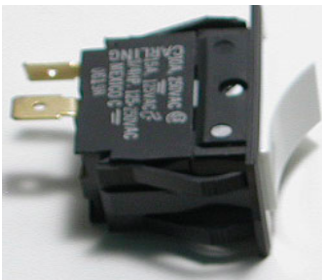
PN: 8536 Switch-Rocker, SPST, On-None-Off, WHT
