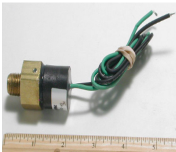
PN: 4669 Switch-Low Pressure, 40 PSI, Air Ride
