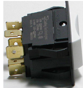
PN: 8607 Switch-Rocker, DPDT, On-Off-On, WHT
