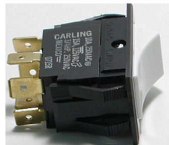
PN: 8563 Switch-Rocker, DPDT, On-None-On, WHT
