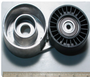
PN: 4713 Assembly Tensioner Arm/Pulley
