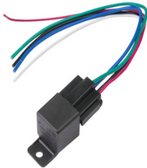
PN: 2443 Harness-ISO Relay/Socket, 12V, 40/60A
