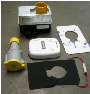
PN: 22203 Shore Power-Auto Eject, 30A, White
