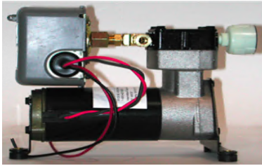
PN: 7678 Compressor 12V, 1.5 CFM, Air Horn
