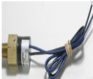
PN: 4668 Switch-High Pressure, 100 PSI, Air Ride
