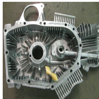
PN: 12129 Cover-Main Bearing, 5.5 Onan
